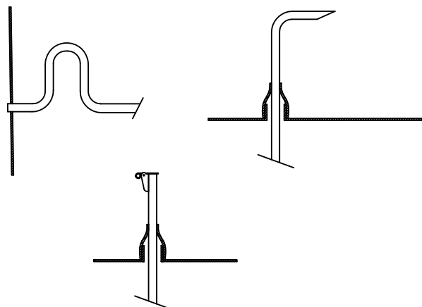
Figure 9. Ways to prevent water to get in
