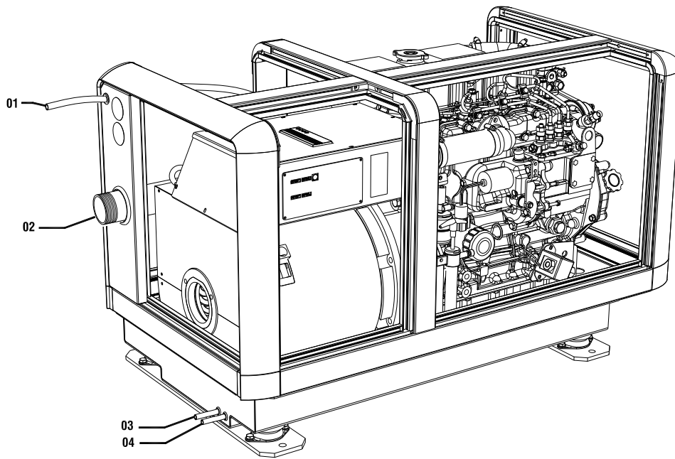
Fig. 15a Connections Whisper 12 Ultra
