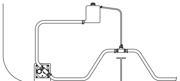
Figure 7: Ventilating an air trap
