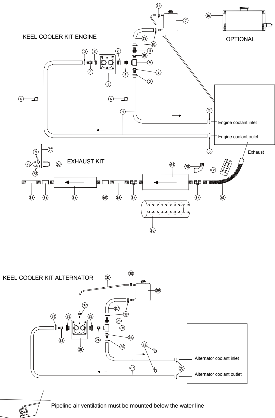
Figure 20: Installation kits
