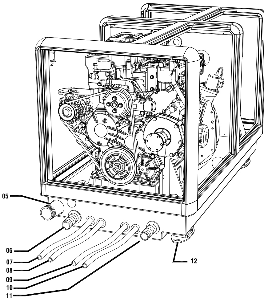
Fig. 17b Connections Whisper 25 Ultra
