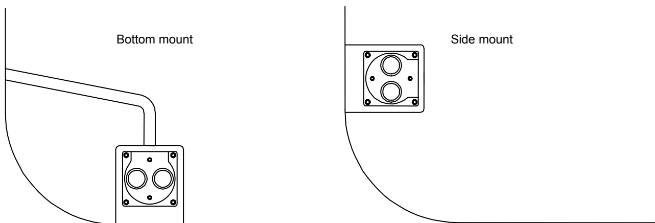
Figure 3: Bottom mount and side mount box cooler
