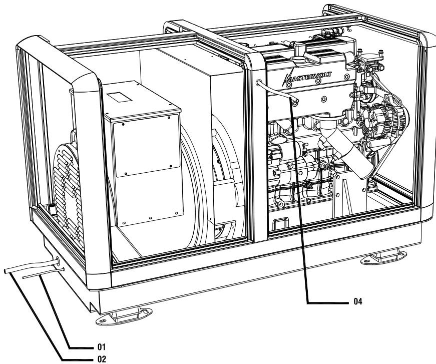
Fig. 17a Connections Whisper 25 Ultra
